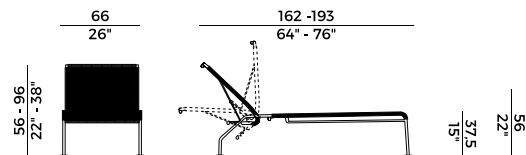
688/D-RECL lettino \ sun lounger
